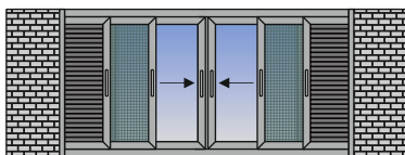
Double sliding pocket sash meeting stile with flyscreen & shutter
